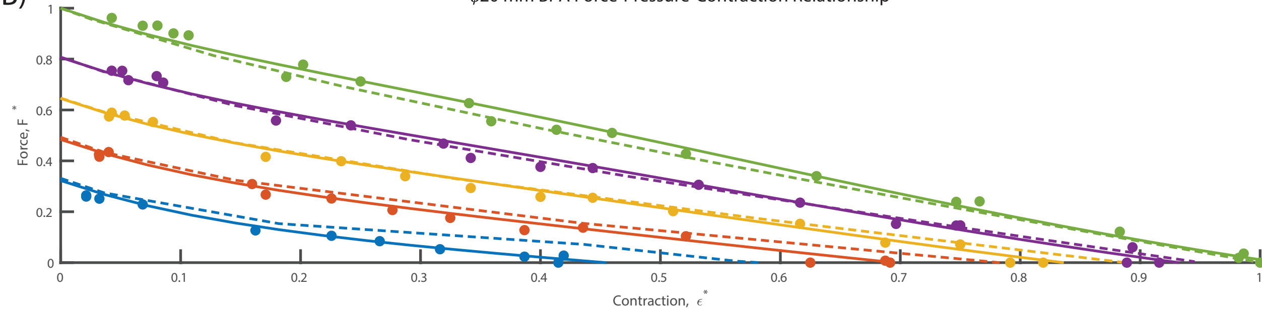
\phi 20 mm BPA Force-Pressure-Contraction Relationship
