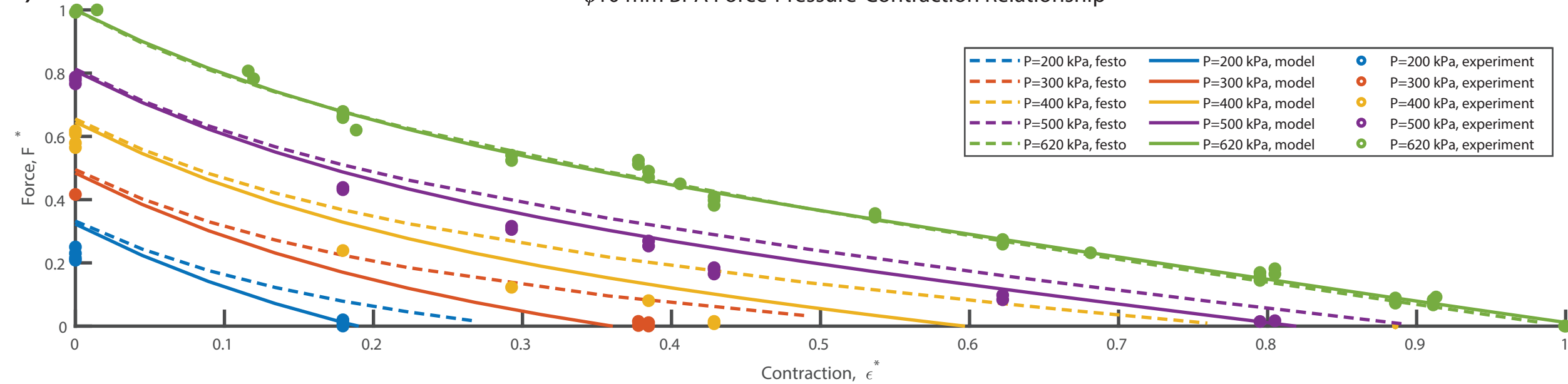
\phi 10 mm BPA Force-Pressure-Contraction Relationship
